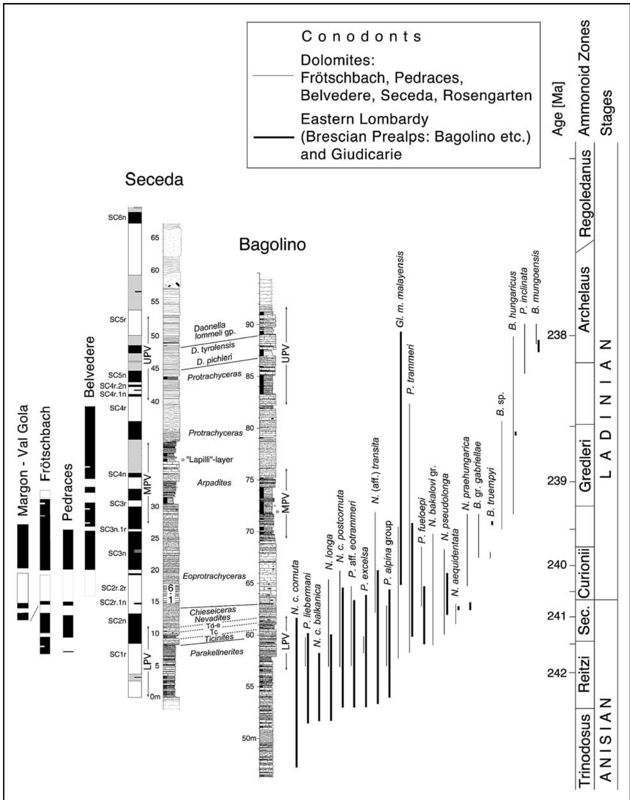
Fig. 8. Integrated Anisian-Ladinian boundary stratigraphy and biochronology. Biostratigraphic data from the Dolomites are projected onto the Seceda outcrop reference stratigraphy, while those from the Brescian Alps and Giudicarie are projected onto the Bagolino reference stratigraphy. Numerical ages are derived from interpolation of dates from Mundil et al. (1996). For details, see Muttoni et al. (2004a) and references therein.
