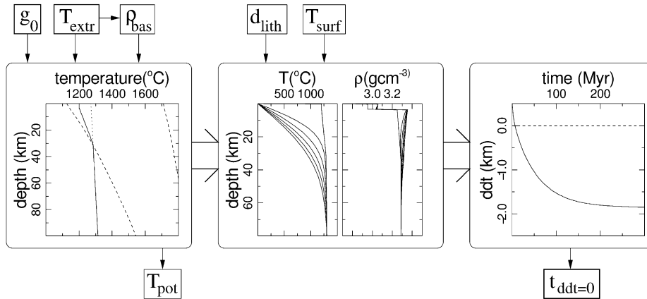
Fig. 1. Experimental setup. From a prescribed magma extrusion temperature (which also gives the crustal density through Eq. (3)) and gravitational acceleration, a geotherm, material stratification (crust + depleted root) and corresponding density profile are calculated. Using a prescribed lithosphere thickness as the extent of the domain for numerical calculation of the time dependent geotherm and using a prescribed surface temperature, the development of the geotherm is integrated in time and corresponding time dependent density profiles are computed. The development of corresponding the density defect thickness, calculated using expression (1), is thus evaluated as a function of time and the zero buoyancy age is found.
