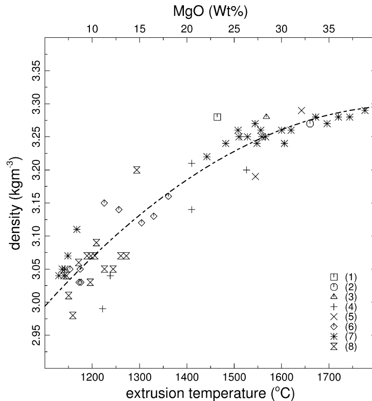
Fig. 2. Primitive magmatic rock densities as a function of MgO content or extrusion temperature, of 58 basalts, komatiitic basalts, komatiites and a picrite. The quadratic best fit for the entire set (see Eq. (3)) is shown by the dashed curve. References for the data are: (1) Parman et al. (1997), (2) Green et al. (1975), (3) Smith et al. (1980), (4) Ludden and Gelinis (1982), (5) Nishihara and Takahashi (2001), (6) Kerr et al. (1996), (7) Puchtel et al. (1998) and (8) Arndt and Nesbitt (1982).
