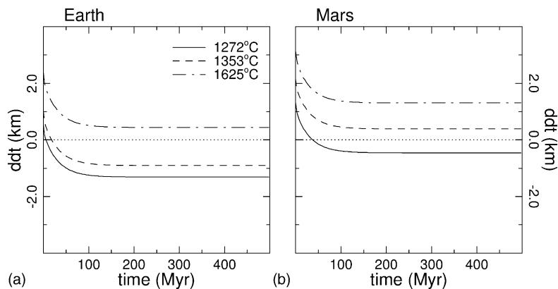
Fig. 4. Density defect thickness time series for the Earth (a) and Mars (b) for potential mantle temperatures of 1272 °C (solid curves), 1353 °C (dashed curves) and 1625 °C (dash-dotted curves). For positive values of the d.d.t. the oceanic lithosphere is buoyant.
