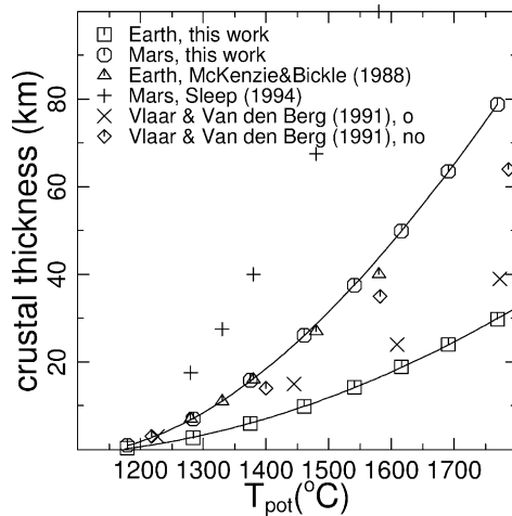
Fig. 3. Thickness of the crust as produced at mid-ocean ridges, for Earth and Mars. The results of McKenzie and Bickle (1988) do not include the effect of the overburden pressure of the crust, and therefore give an overestimate of the thickness. The results for Mars by Sleep are those of McKenzie and Bickle (1988) divided by a factor of 0.4 to correct for different gravity and a somewhat more iron-rich composition of the basalts (Sleep, 1994). The results of Vlaar and Van den Berg (1991), with (o) and without (no) including the effect of the crustal overburden, clearly show that the crustal overburden is an important effect which should not be neglected.
