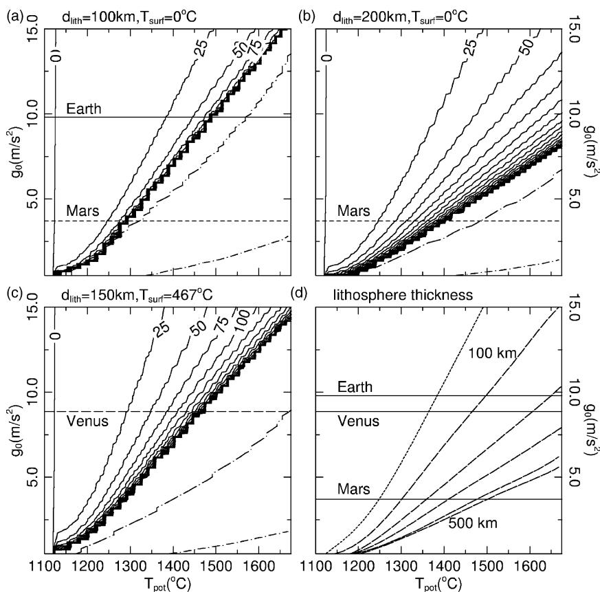
Fig. 5. Frames a–c show contours of the neutral buoyancy times (density defect thickness = 0). (a) Surface temperature is 0^\circ\text{C} and lithosphere thickness is 100 km, potentially applicable to both Earth and Mars. The gravitational accelerations for these terrestrial planets are included as horizontal lines (solid: Earth, dashed: Mars). (b) Surface temperature is 0^\circ\text{C} and lithosphere thickness is 200 km, potentially applicable to Mars, including the gravitational acceleration of Mars (dashed line). (c) Surface temperature is 467^\circ\text{C} and lithosphere thickness is 150 km, potentially applicable to Venus, including the gravitational acceleration of Venus (long-dashed line). (d) Variation of neutral buoyancy times as a function of lithosphere thickness for a surface temperature of 0^\circ\text{C} . Acceleration of gravity values for Earth, Venus and Mars are indicated by solid lines. The 25 Myr isoline (approximately coinciding for all values of the lithosphere thickness applied) is indicated by the dotted curve. Dashed curves indicate the position of the 500 Myr isoline for lithosphere thicknesses of 100, 150, 200, 300 and 500 km.
