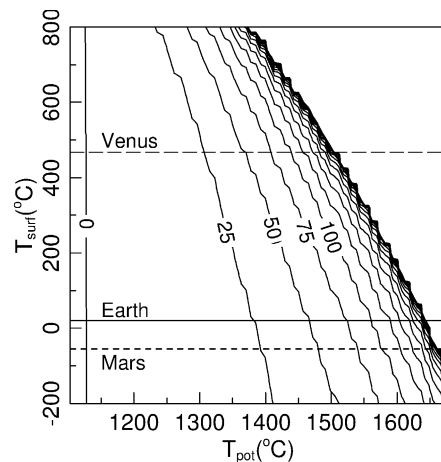
Fig. 6. Neutral buoyancy times (density defect thickness = 0) ranging from 25 to 500 Myr for a constant gravitational acceleration of 9.8 \text{ ms}^{-2} and lithosphere thickness of 150 km as a function of potential temperature and surface temperature. The horizontal lines indicate the position of Venus (long-dashed), Earth (solid) and Mars (dashed).
