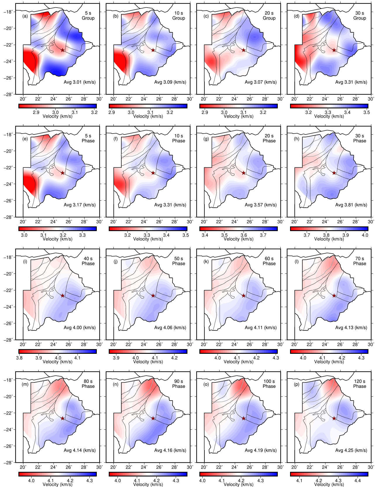
Figure 2. (a–d) Group and (e–h) phase velocity maps from ambient noise tomography for periods of 5 to 30 s. (i–p) Phase velocity maps from Helmholtz tomography for periods of 40 to 120 s. The red star indicates the location of the 3 April 2017 earthquake.
