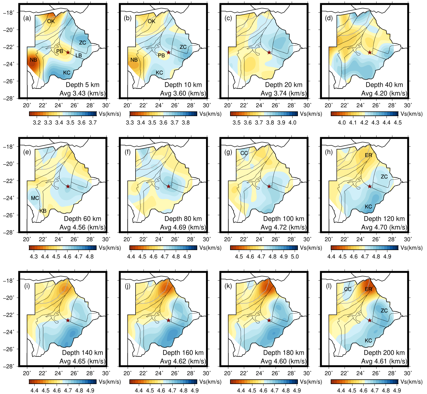
Figure 3. (a–l) Depth slices of absolute shear wave velocity through the 3-D model. The red star indicates the location of the 3 April 2017 earthquake. CC = Congo Craton; ER = East African Rift System; KB = Kheis Belt; KC = Kaapvaal Craton; LB = Limpopo Belt; MC = Maltahohe Craton; NB = Nosop Basin; OK = Okavango Rift Zone; PB = Passarge Basin.
