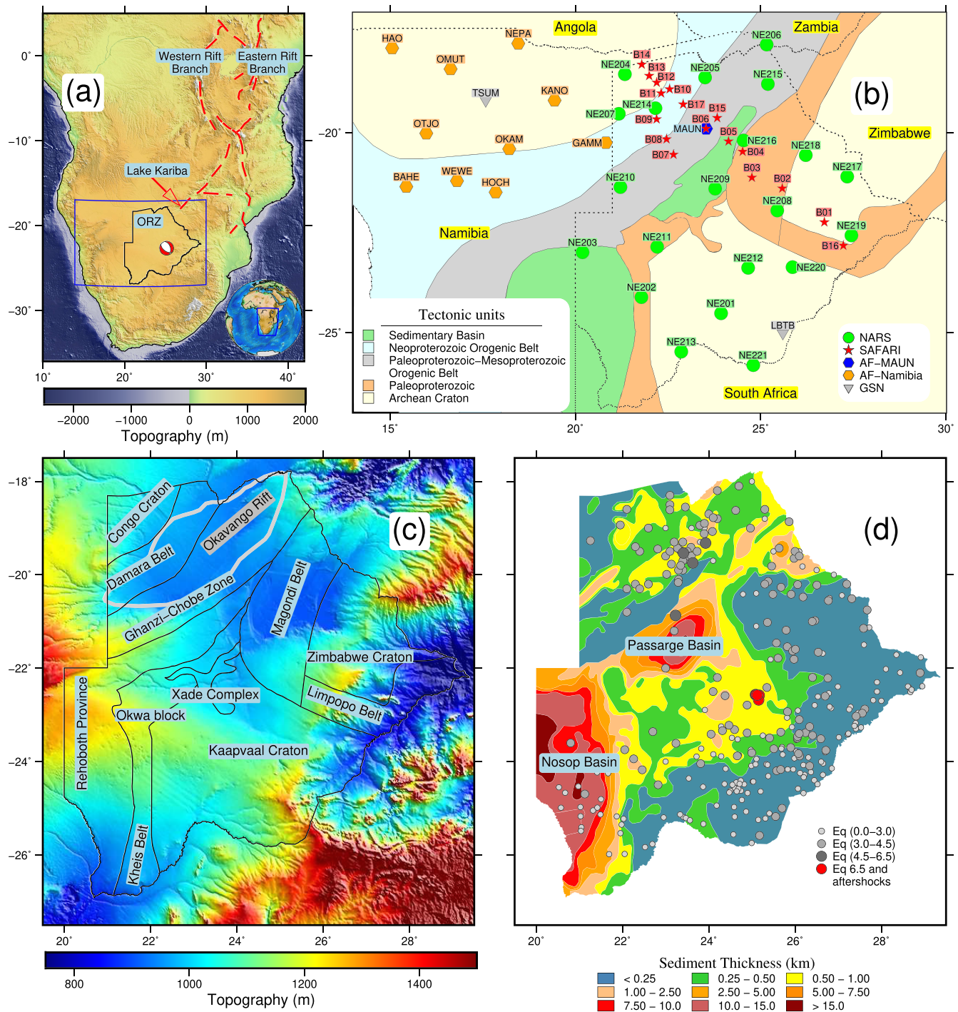
Figure 1. (a) Topography of southern Africa with the branches of the EARS (Chorowicz, 2005), Lake Kariba, the focal mechanism of the 3 April 2017 earthquake and outlines of Botswana and Figure 1b. (b) Tectonic map of the region with the distribution of seismic stations. (c) Tectonic units of the study area (Okavango Rift Zone with gray outline). (d) Sedimentary thickness map from aeromagnetic data after Pretorius (1984) and earthquake distribution. The 3 April 2017 earthquake and its aftershocks are shown in red.
