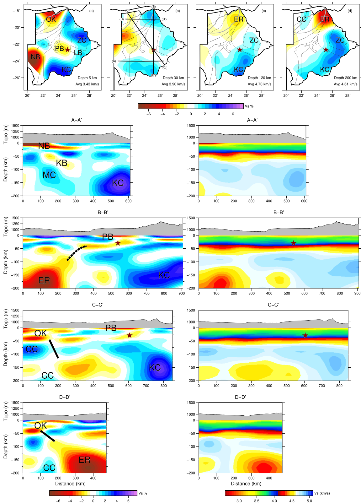
Figure 4. The 3-D shear wave velocity model of Botswana. (a–d) Relative velocity maps at 5, 30, 120 and 200 km depths, respectively. The black lines in (b) show the locations of the cross sections. The red star indicates the location of the 3 April 2017 earthquake. The cross sections are shown in relative (left) and absolute (right) shear wave velocity to highlight the subsurface structures that are discussed in the text. CC = Congo Craton; ER = East African Rift System; KB = Kheis Belt; KC = Kaapvaal Craton; LB = Limpopo Belt; MC = Malthaho Craton; NB = Nosop Basin; OK = Okavango Rift Zone, PB = Passarge Basin.
