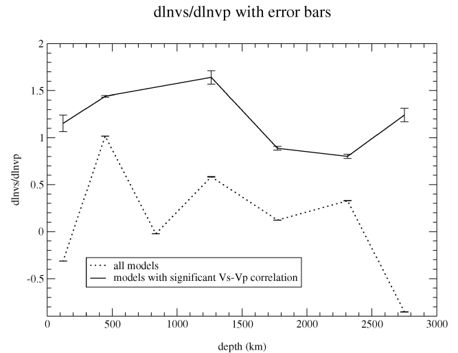
Figure 11. Ratio between degree two d \ln V_s and d \ln V_p as a function of depth.
