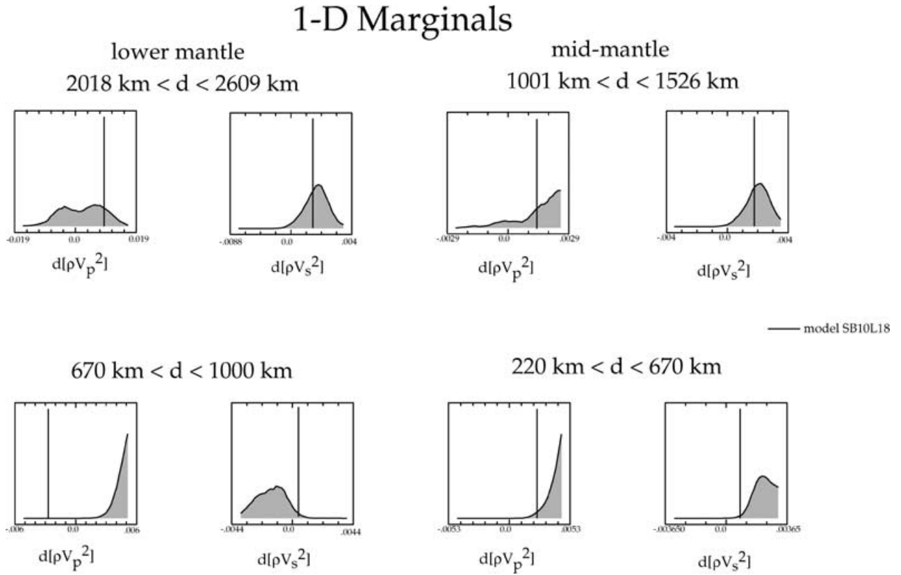
Figure 5. 1-D marginals corresponding to the real part of c_2^1 ( \delta c_2^1/c ). The vertical black line is the position of model SB10L18. The full range of the models space is shown.
