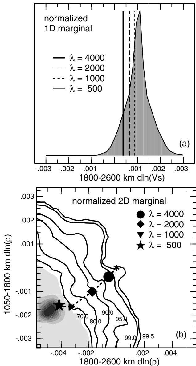
Figure 3. Comparison of results for NA ‘mapping’ and damped least-squared inversions applied to data set 1 for degree-two zonal structure. This experiment employs real data rather than synthetics, in an inversion for three velocity and four density parameters. (a) The NA Bayesian 1D marginal likelihood for deep-mantle v_s , which corresponds to a diagonal element of the inversion covariance matrix, together with values obtained from least-squared inversions with four damping values. Larger \lambda implies stronger damping. A wide range of damping values all give results within the high-likelihood region, and weaker damping moves the result closer to the likelihood peak. (b) An NA Bayesian 2D marginal likelihood for two density parameters, which corresponds to an off-diagonal element of the covariance matrix, again shown with results from several damped inversions. Increasing likelihood is shown with darker shading. The lower likelihood contours are shown as confidence levels (confidence increases with the total enclosed likelihood). Weaker damping moves the inversion results from the starting model (the asterisk at the centre) along a ‘ridge’ toward the likelihood peak.
