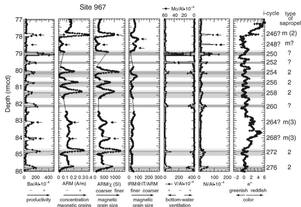
Figure M53 A series of geochemical and magnetic proxies measured on samples from ODP Site 967 (Eastern Mediterranean) with their meaning underneath the abscissas (after Larrasoana et al. , 2003a). Sediments constitute an alternation of marly limestones and marls with sapropels intercalated (sapropels are sediments with more than 2% organic matter and therefore dark-brown to black colored). Sapropelic sediments are indicated by darkest gray shading, dissolution zones with intermediate gray, and reoxidized zones with lightest gray. The insolation cycle (i-cycle) codification implies an age range from ~2.9 to ~2.5 Ma. The sapropels class into groups (2) and (3). Arrows indicate the position of completely reoxidized (missing, m) sapropels on the basis of magnetic and geochemical proxies. In cases where assignment to a sapropel type is not certain because of lack of magnetic data due to unavailability of the core segment for rock magnetic analysis, a question mark is put.
