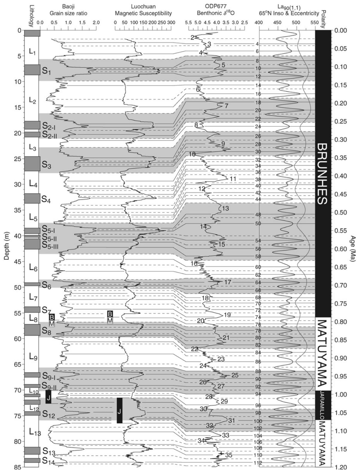
Figure M52 Correlation of the Baoji grain-size ratio ( <2 \mu\text{m} / >10 \mu\text{m} ) and Luochuan low-field magnetic susceptibility ( \chi_{in} ; fitted to the Baoji depth scale) to the 65°N insolation curve of Laskar (1990) (i-cycle numbers shown on the left) and the ODP677 benthonic \delta^{18}\text{O} record (Marine isotope stages adjacent to curve). The eccentricity component from the Laskar (1990) solution is displayed for comparison with the longer term trends observed within the loess record. Correlation points linking warm features are shown with full lines while those for cold features are shown with dashed lines.
