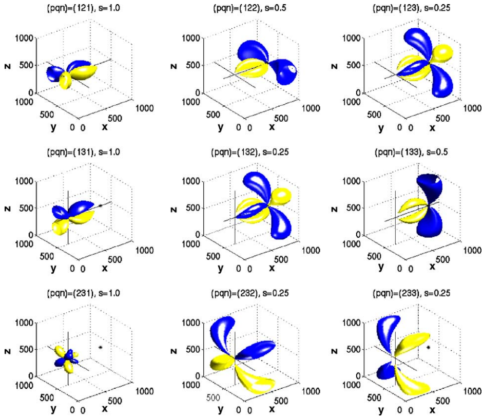
Fig. 2. Iso-surfaces of the sensitivity kernels -a_{pq}^{FFF} \cdot b_n^{FFF} plotted at values of \pm s \cdot [(600 \text{ km})^2 \cdot (4\pi\alpha^3) \cdot (4\pi\alpha^2)]^{-1} , where the scaling factor s is given in the sub-figure captions. Yellow (gray in the print edition) denotes positive and blue (black in the print edition) negative values. Wave speeds are \alpha = 5 \text{ km s}^{-1} and \beta = \alpha/\sqrt{3} \text{ km s}^{-1} . The source is located at (x, y, z) = (200, 500, 500) \text{ km} and the receiver, marked by a star (*), is at (x, y, z) = (800, 500, 500) \text{ km} . Black lines intersecting at the source indicate the (pq) -plane. The index n represents the observation direction. The sensitivity kernels plotted in the first row ((1, 2)-couple) have expected correspondences in the second row ((1, 3)-couple). It is noteworthy that there are significant sensitivity contributions between source and receiver only if one of the two source dipoles points towards the receiver. Therefore, in the case of the (2, 3)-couple the sensitivities practically vanish in the region between source and receiver. Large sensitivity contributions in regions behind source or receiver and far away from the line connecting source and receiver arise if the observation direction n does not point toward the source.
