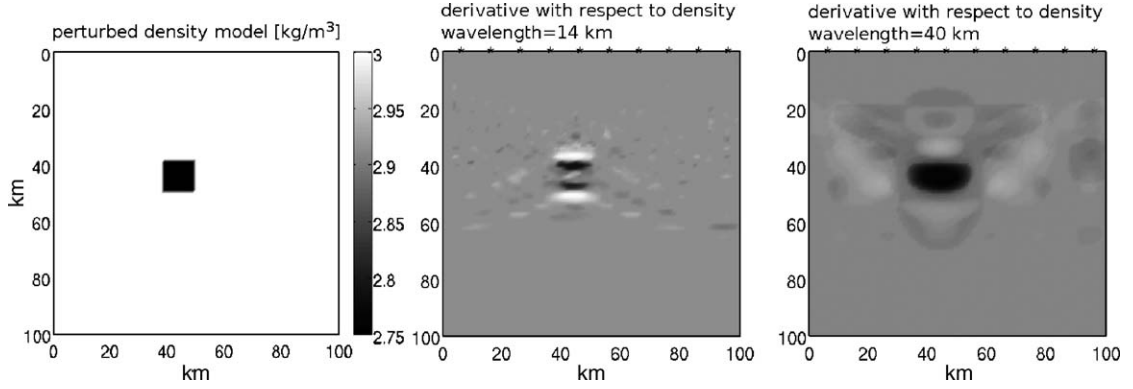
Fig. 1. Left : Perturbed density model. The reference model is homogeneous in both density and shear modulus ( \rho = 3.0 \times 10^3 \text{ kg m}^{-3} , \mu = 75.0 \times 10^9 \text{ N m}^{-2} ). There are no shear modulus perturbations. Middle : Derivative of the objective function \mathcal{E} with respect to density for a dominant signal wavelength of \lambda_0 = 14 \text{ km} . Only the edges of the perturbation are mapped by D_\rho \mathcal{E} . The interior of the density perturbation remains invisible. (The gray-scale values apply only to the figure on the left because the amplitude of the derivatives are proportional to the amplitudes of the signal.) Right : D_\rho \mathcal{E} for \lambda_0 = 40 \text{ km} . Since the wavelength is longer, the entire density perturbation acts as a scatterer. It therefore maps as one single object into the derivative.
