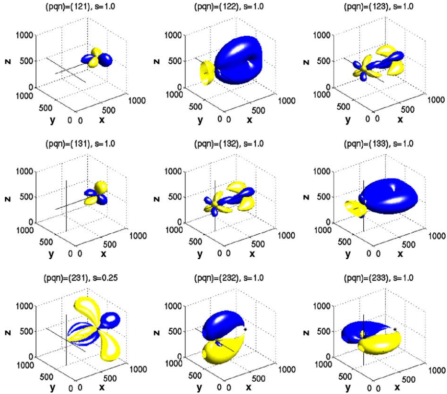
Fig. 5. The same as Fig. 2 but for the sensitivity kernels -\mathbf{a}_{pq}^{SFF} \cdot \mathbf{b}_n^{SFF} plotted at values of \pm s \cdot [(600 \text{ km}^2)^2 \cdot (4\pi\rho\beta^3) \cdot (4\pi\rho\beta^2)]^{-1} . The scaling factor s is given in the sub-figure titles. Again, most of the sensitivity densities are concentrated in regions around source or receiver. Significant contributions along the line connecting source and receiver can only be observed in the cases of the (122) and (133) kernels.
