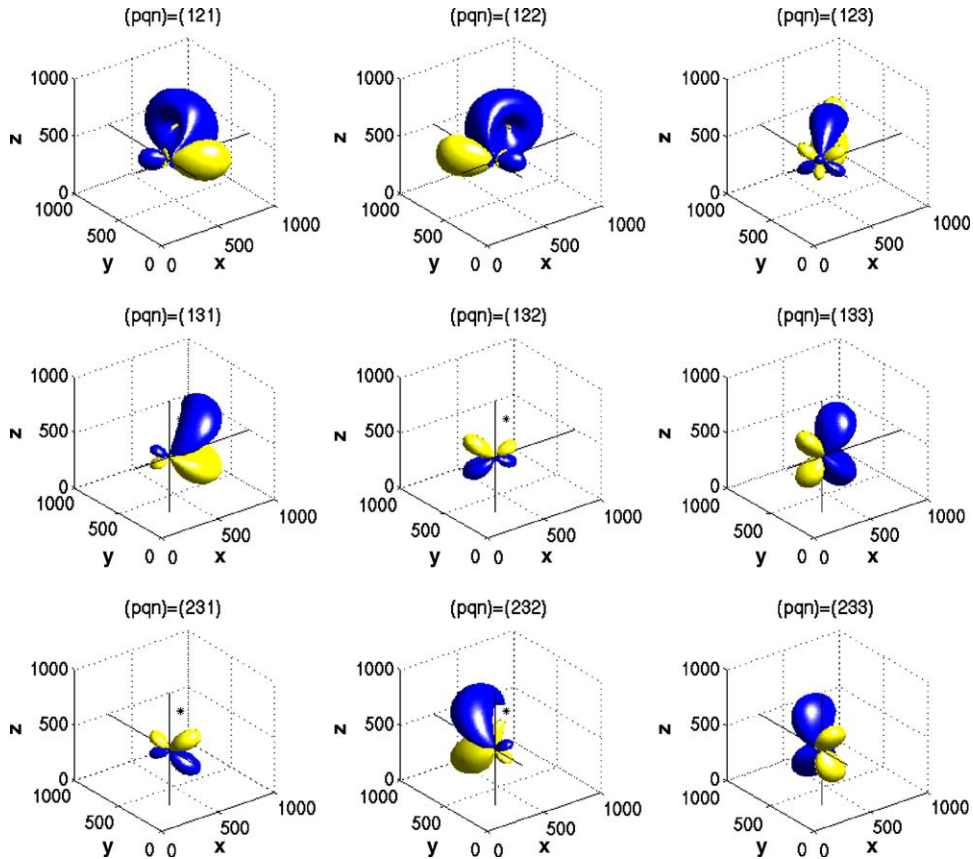
Fig. 6. The same as Fig. 3 but with the source and the receiver located at (x, y, z) = (300, 300, 500) km and (x, y, z) = (724, 724, 500) km, respectively. Symmetries between the first row ((1, 2)-couple) and the second row ((1, 3)-couple) as observed in Fig. 3 do not exist. In general the sensitivity densities are small in the region between source and receiver. This effect is again especially pronounced in the case of the (2, 3)-couple.
