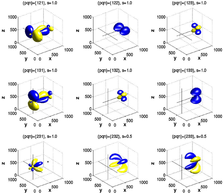
Fig. 4. The same as Fig. 2 but for the sensitivity kernels -\mathbf{a}_{pq}^{SFF} \cdot \mathbf{b}_n^{PFF} (S to P conversions) plotted at values of \pm s \cdot [(600 \text{ km})^2 \cdot (4\pi\rho\beta^3) \cdot (4\pi\rho\alpha^2)]^{-1} . The scaling factor s is given in the sub-figure titles. As expected from the source-receiver asymmetry of the sensitivity kernels, there are no similarities between the S→P kernels and the P→S kernels shown in Fig. 3. Generally, the sensitivity densities are small in the region between source and receiver, the only exceptions being the (121) and the (131) kernel.
