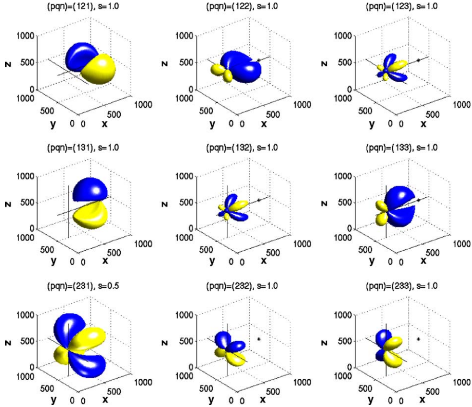
Fig. 3. The same as Fig. 2 but for the sensitivity kernels -\mathbf{a}_{pq}^{PFF} \cdot \mathbf{b}_n^{SFF} (P to S conversions) plotted at values of \pm s \cdot [(600 \text{ km})^2 \cdot (4\pi\rho\alpha^3) \cdot (4\pi\rho\beta^2)]^{-1} . The scaling factor s is given in the sub-figure titles. Symmetries between the first row ((1, 2)-couple) and the second row ((1, 3)-couple) are again due to choosing the line connecting source and receiver as parallel to the x -direction. In general the sensitivity densities are small near the region between source and receiver. This effect is especially pronounced in the case of the (2, 3)-couple, as already observed for the P→P kernels shown in Fig. 2.
